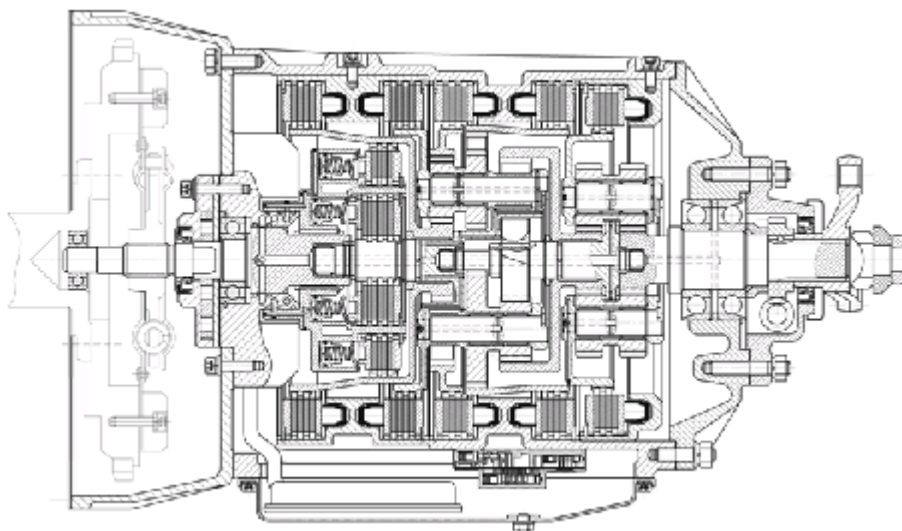
Fig. 3. The design of the eight-speed planetary gearbox on the basis of universal multi-threaded differential mechanism
