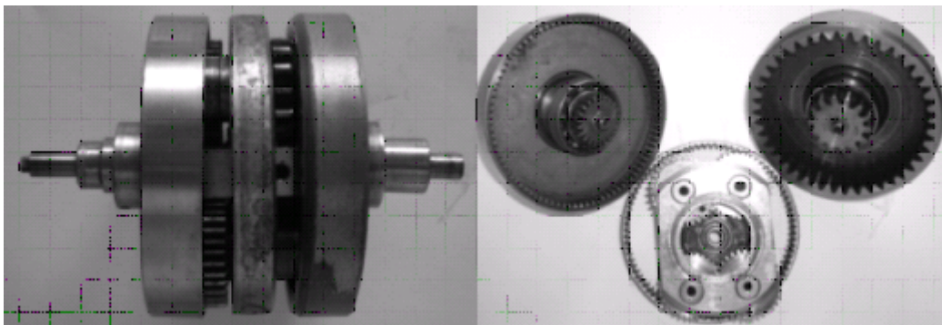
Fig. 1. The design of the planetary system of universal multi-threaded differential mechanism
