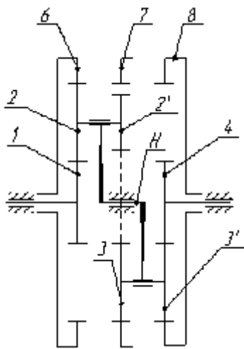
Fig. 2. Kinematic diagram of the eight-speed planetary gearbox
